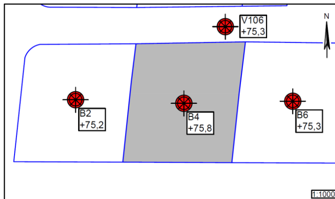
Figur 1 – Situationsplan 1:1000, Hvedebakken 4
