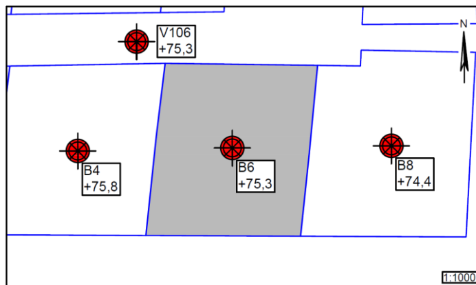
Figur 1 – Situationsplan 1:1000, Hvedebakken 6
