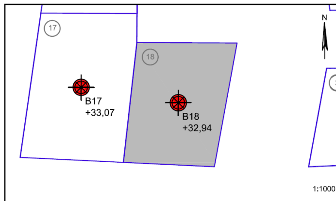
Figur 1 – Situationsplan 1:1000, Parcel nr. 18
