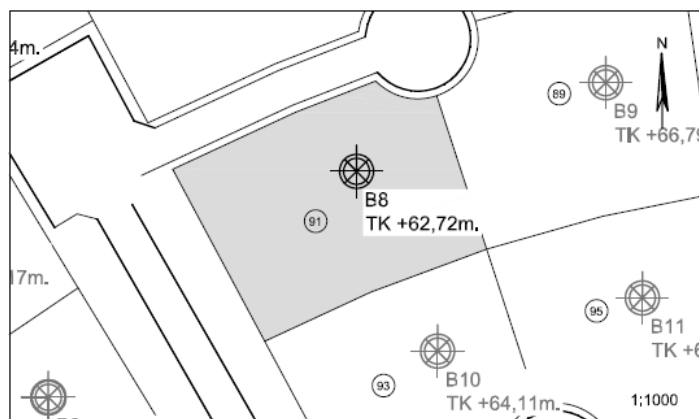
Figur 1 – Situationsplan 1:1000, Parcel nr. 91
